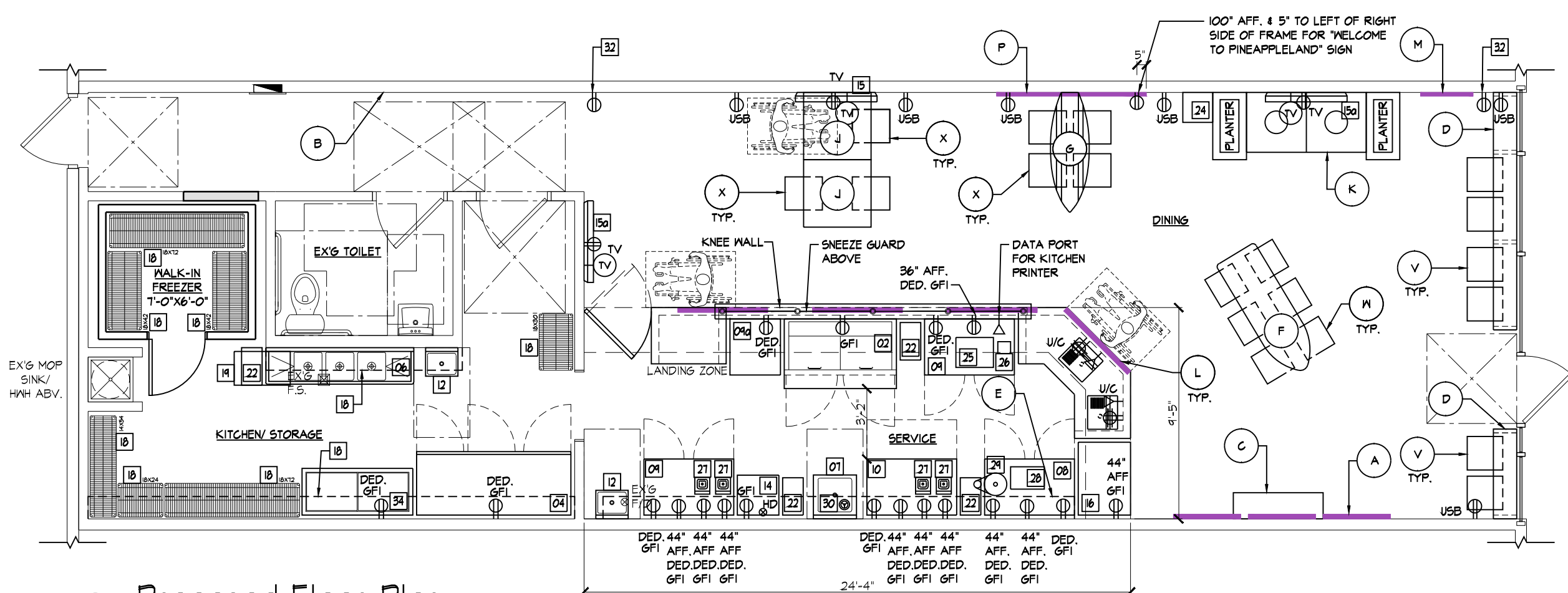
1 Proposed Floor Plan 3/16"=1'-0" REVISION 6
